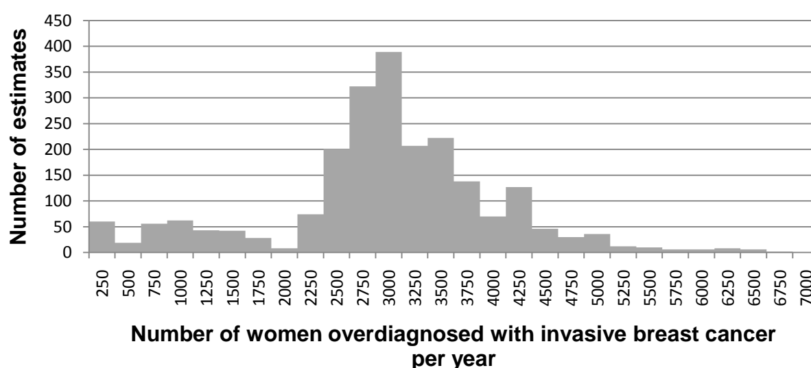
Figure 2 Histogram of the range of estimates
